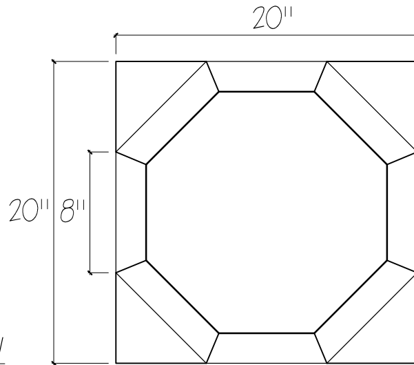
Plan/ Top View
